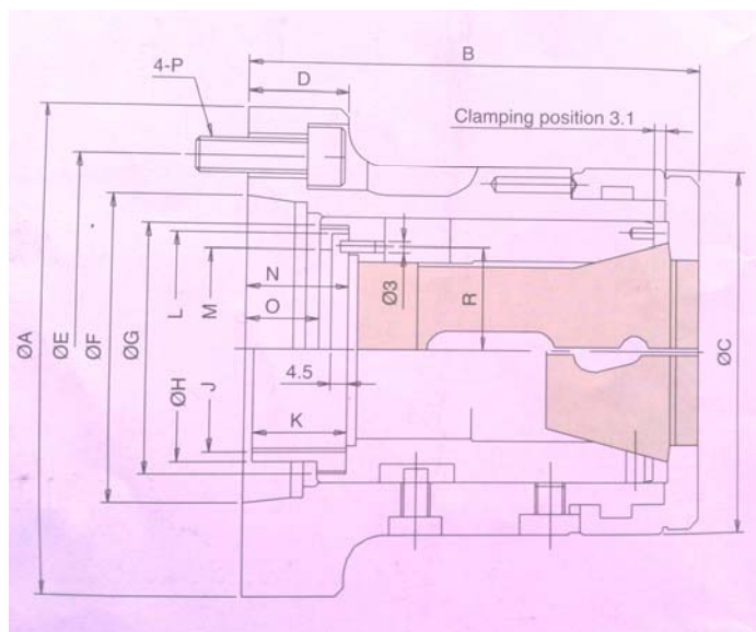
Spring Collet
