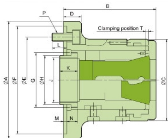
Spring Collet
